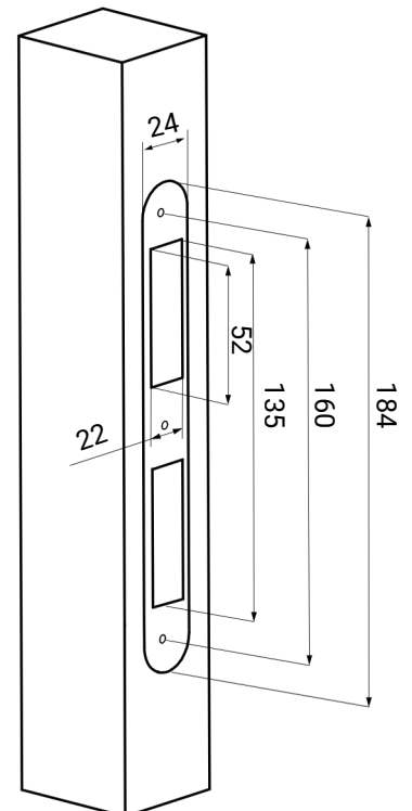
Frame strike plate (G0320)
